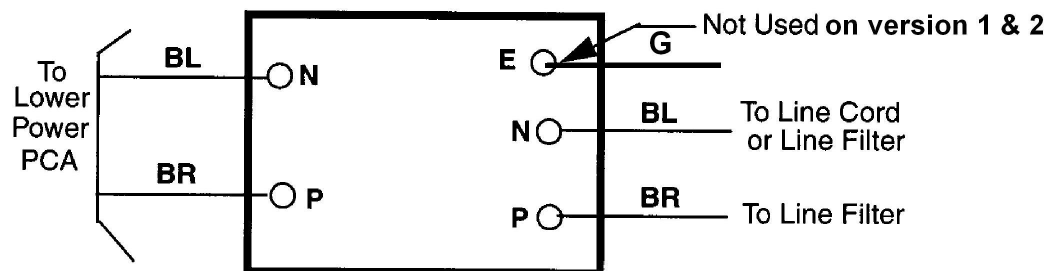
Diagram 6.13 ó Line Filter Wiring
